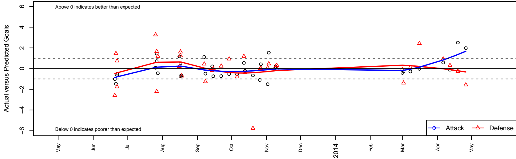
BSC Portland Black II G00 Dots are actual minus expected GF (blue circles) and GA (red triangles). Blue line is smoothed change in attack strength. Red is smoothed change in defense strength.
